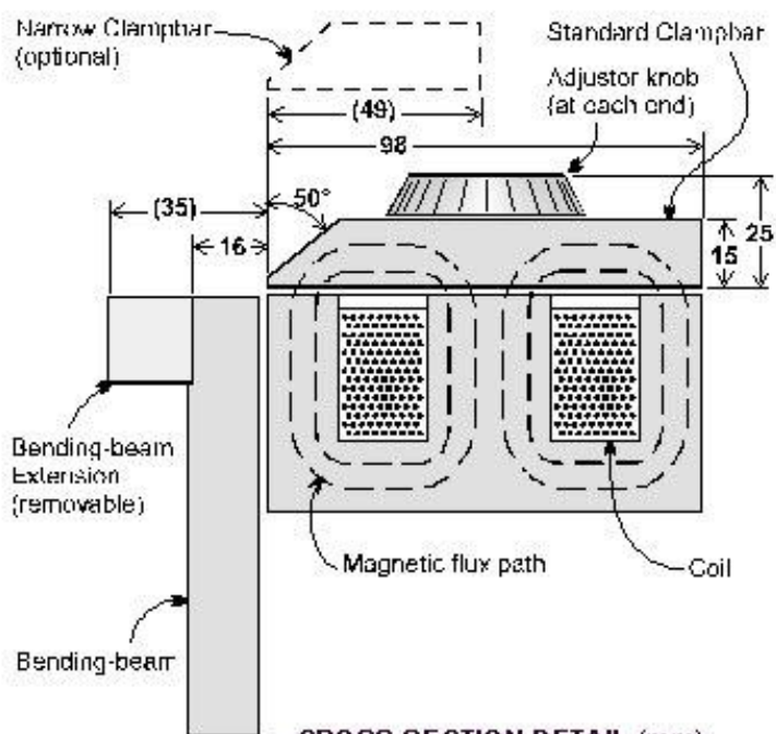
CROSS-SECTION DETAIL (mm)
